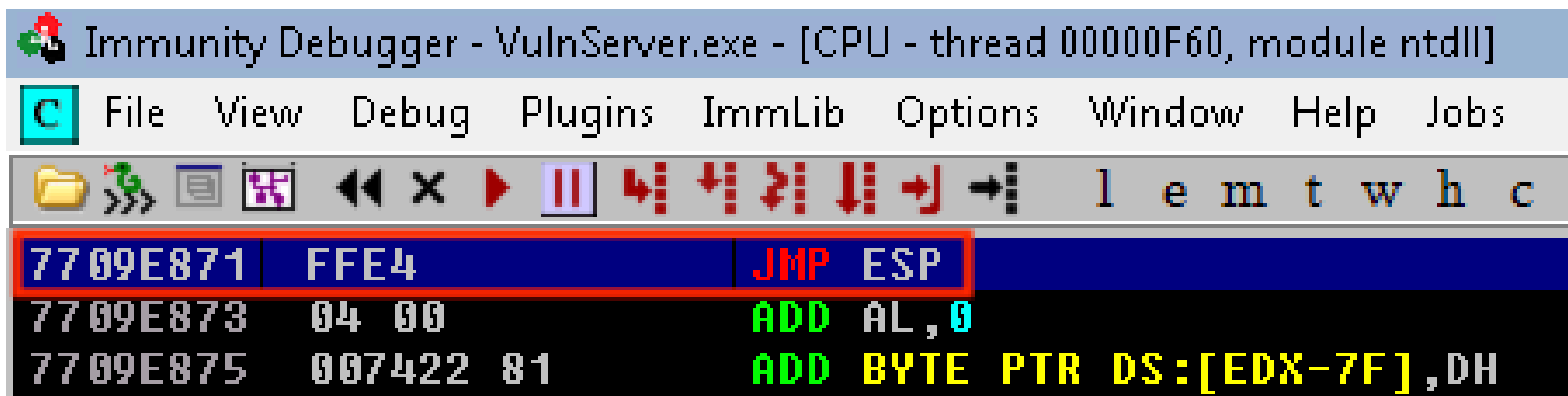
Figure 138: Impermanent JMP ESP instruction located at 7709E871, pre-restart
