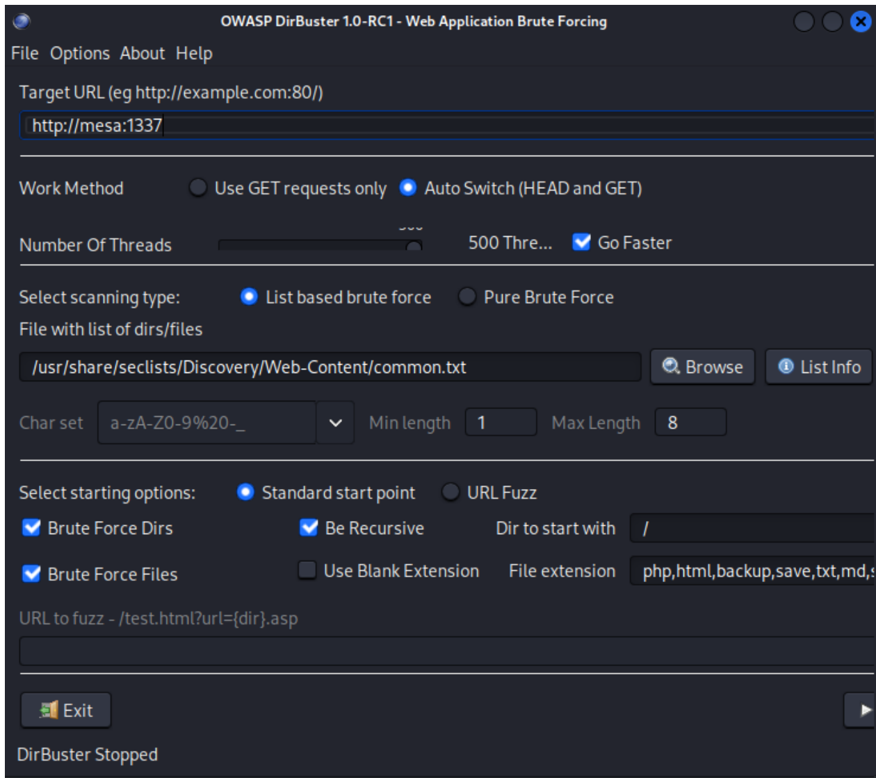
Figure 146: Port 1337 scan - Dirbuster setup
